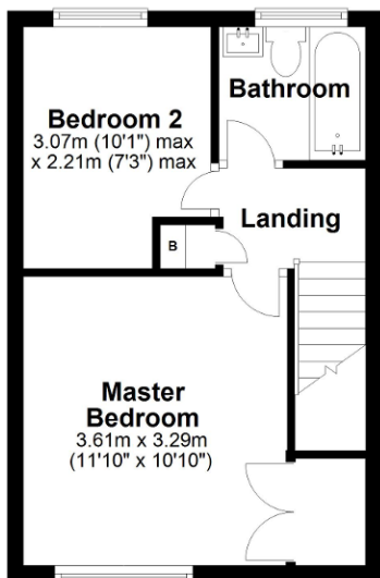
First Floor Approx. 21.3 sq. metres (229.6 sq. feet)
